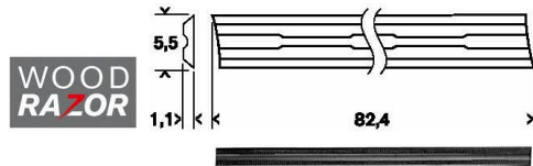
fer woodrazor
